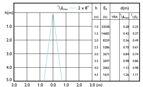
LED PAR30L 28W 15D 100-277V
