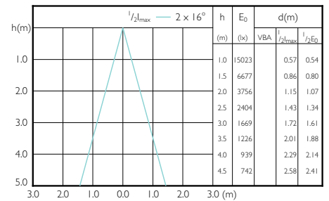
LEDspot MAS 41W E27 PAR30L 830 30D ND
