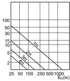
SDAC_LEDspotL_0138-Accent diagram
