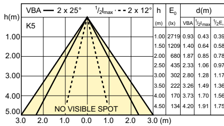
SDBE_LEDspotL_0132-Beam diagram
