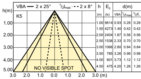
SDBE_LEDspotL_0144-Beam diagram
