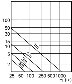
SDAC_LEDspotL_0135-Accent diagram
