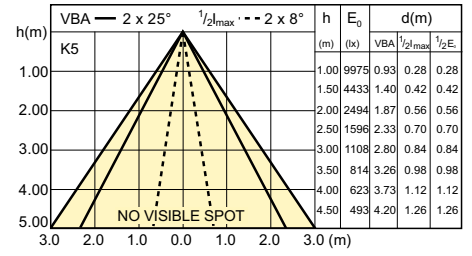
SDBE_LEDspotL_0143-Beam diagram
