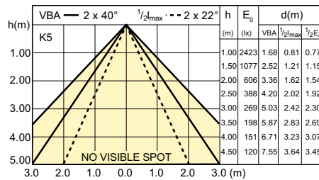
SDBE_LEDspotL_0142-Beam diagram
