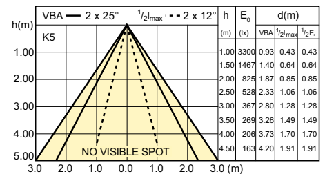
SDBE_LEDspotL_0137-Beam diagram
