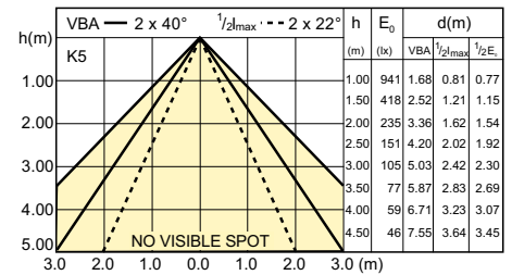
SDBE_LEDspotL_0134-Beam diagram
