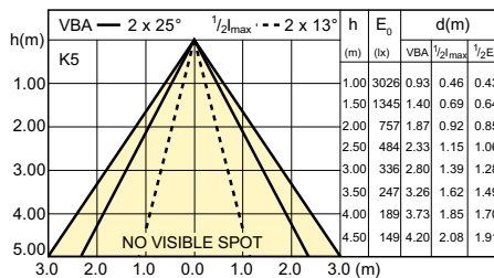
SDBE_LEDspotL_0136-Beam diagram
