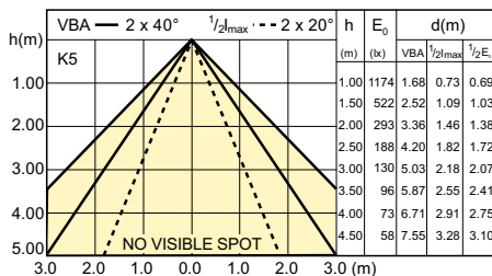
SDBE_LEDspotL_0135-Beam diagram
