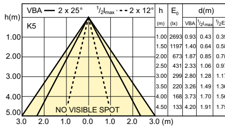
SDBE_LEDspotL_0133-Beam diagram
